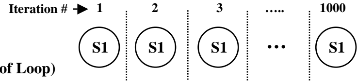
Dependency Graph
